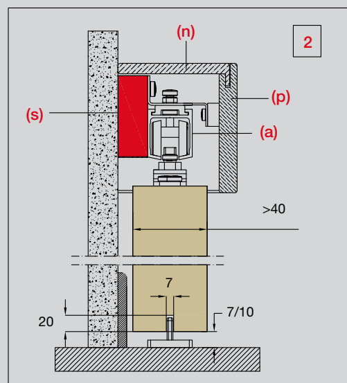
B) Installazione a parete con zoccolino, per pannelli con spessore (SP) > 40 mm. Installation with skirting board, for door panels of (SP) > 40 mm thick.
