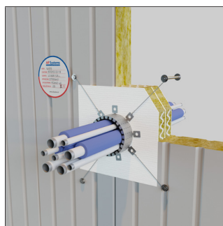
Parete Sandwich
