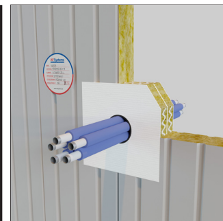
Parete Sandwich
