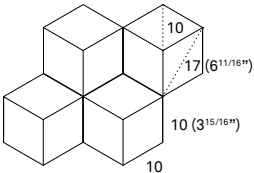
MOSAICO ROMBI ◆ 30,5x35,2 (12 1/16"x13 7/8") RT 9 mm
