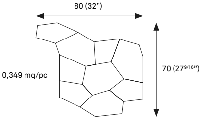
DECORO IDRO BEAT CELL ● 70x80 (27 9 / 16 "x32") RT 9 mm
