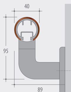
Mensola in Acrovyn®
