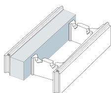
BIOPLUS 50 H10 cm LxHxsp: 500x100x335 mm
