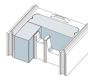
BIOPLUS JOLLY MEZZO H10 cm LxHxsp: 250x100x335 mm
