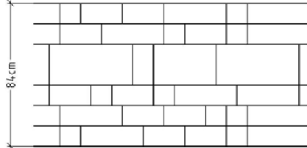
TIPO 111 H12: 72% (5/7) H24: 28% (2/7)
