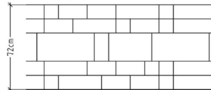
TIPO 112 H12: 25% (1/4) H24: 75% (3/4)
