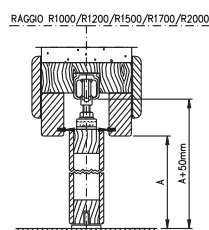
Porta anta unica destra /Right single door
